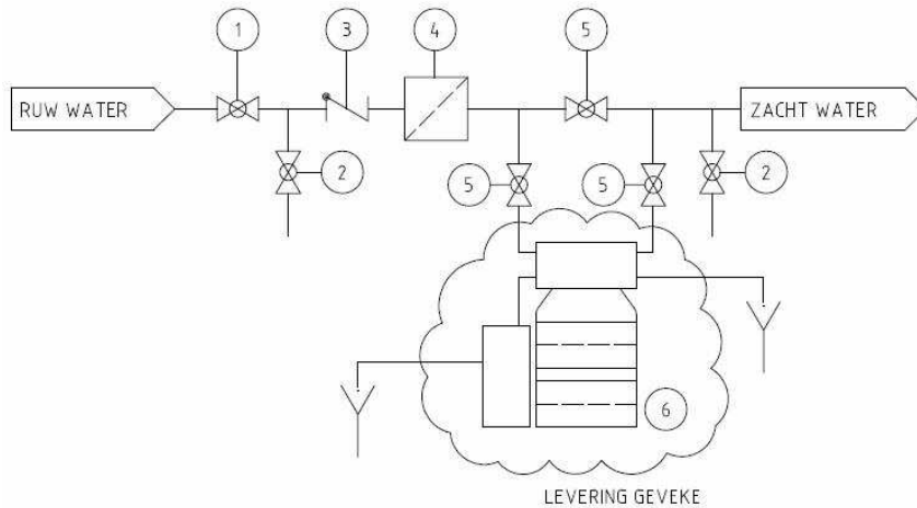
Installatieschema CondairSoft 070S t/m 100S
